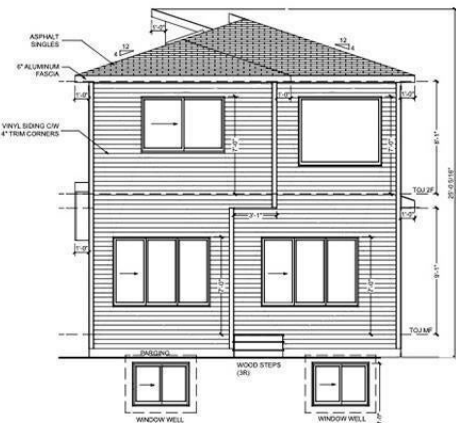
REAR ELEVATION
